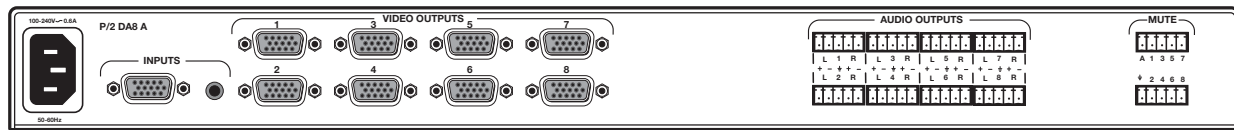
P/2 DA8 A - Back
